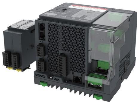
PowerLogic ION9000 bottom with two option modules
