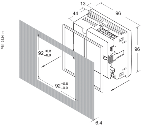
Dimensions PM5350IB
