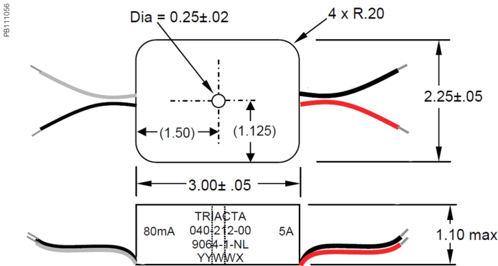
The 5 A to 80 mA converter dimensions
