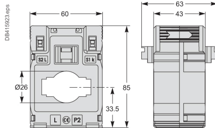
MC internal profile type
